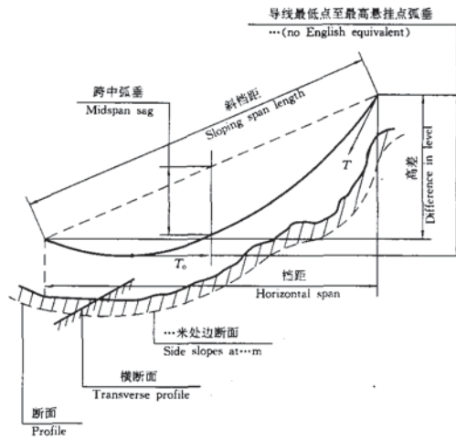
SLOPING SPAN
