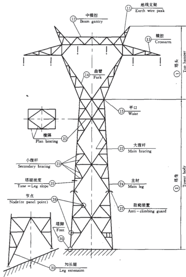
LATTICE TOWER
