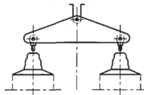
Yoke plate 图9 联板
